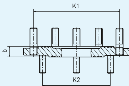
Studded reducer flange XR 200/200 Type A - PN16/PN10 (12 x 8 bolt holes)
