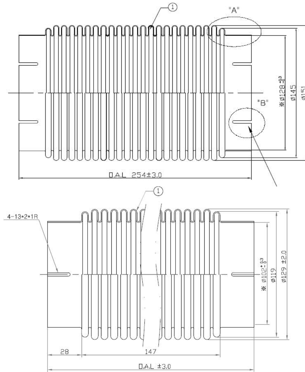
Above : Examples of Stainless Steel Exhaust Expansion Joint
