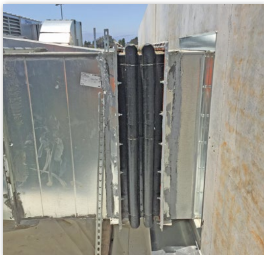
ME-2, 2 Arch Rectangular Duct Connector installed.
