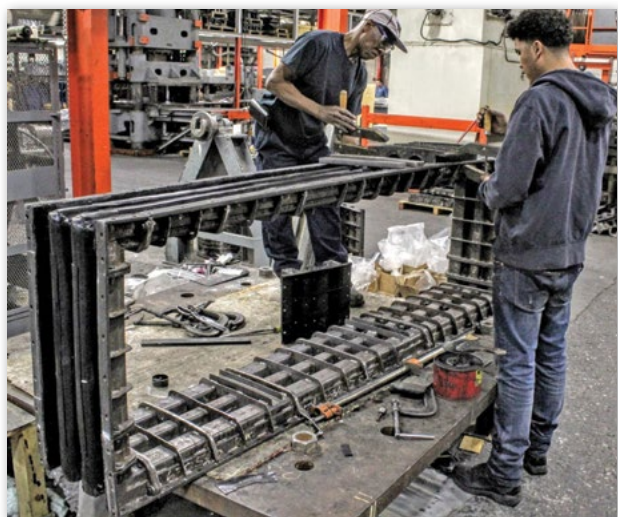
Building an ME-2 2 Arch Rectangular Duct Connector in the Mercer Plant. All steel forms are made by Mercer to your requirements.
