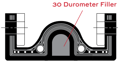
OPTIONAL FILLED ARCH CONSTRUCTION
